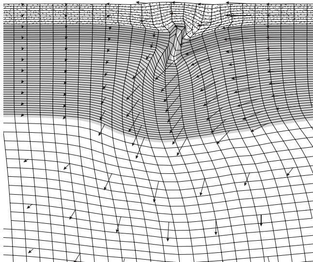
(a) \Delta x = 100 km
