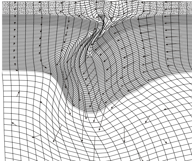
(b) \Delta x = 150 km
